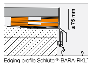
Edging profile Schlüter®-BARA-RKLT
